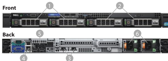
1. 2x 2.5" SSD for OS (RAID-1) | 2. 2x Empty Drive Bays | 3. 2x 1GbE | 4. 2x 1GbE | 5. Management Module | 6. 2x Redundant Hot-Plug Power Supplies
