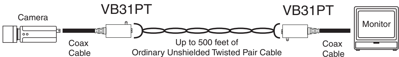
Basic Twisted Pair Video Transmission System
