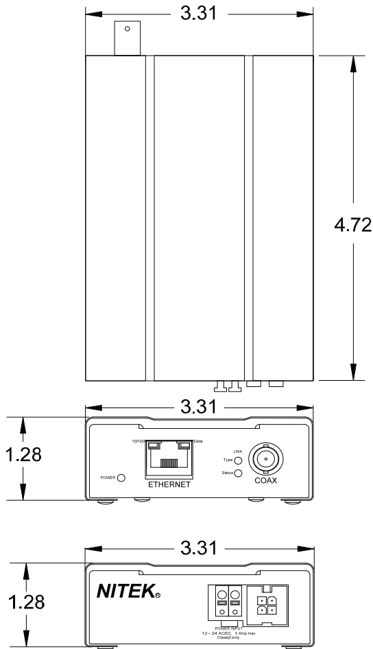
VR448COAX Receiver
