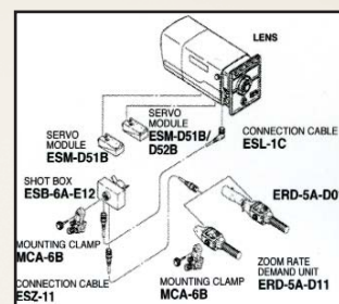
SS-23D (Shot Box w/Focus Demand)
