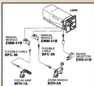
SS-21D Servo Zoom / Servo Focus
