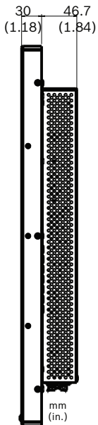
UML-323-90: Side View
