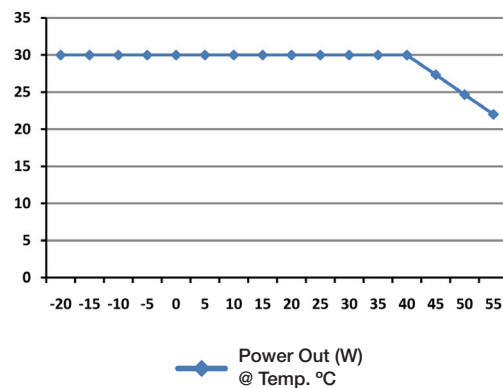
PD-9001GR Performance
