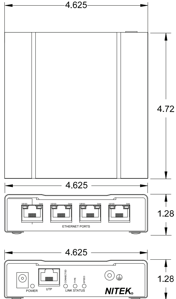
VR448UTP Transmitter w/PoE
