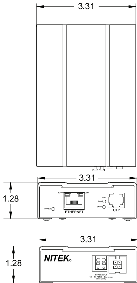
VR448UTP Receiver
